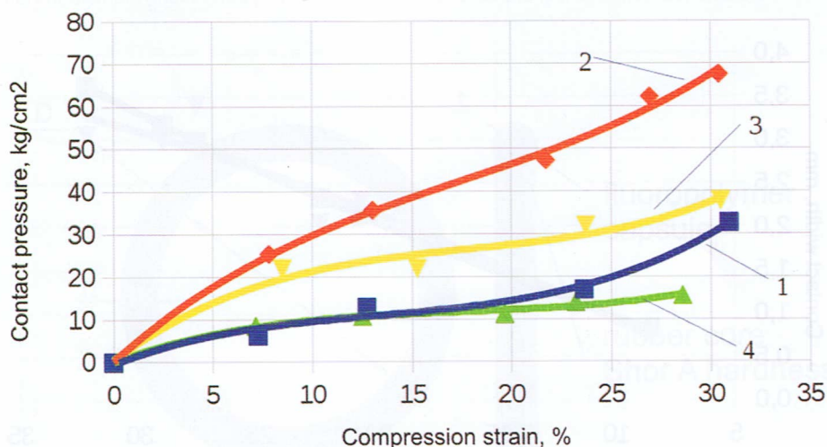
Figure 6. Contact pressure vs compression strain for encapsulated rings with a cross-sectional diameter of 5.8 mm and different core hardnesses and capsule thicknesses: 1, 2 — core hardness Shor A 70; 3, 4 — core hardness Shor A 55; 2, 3 - capsule thickness 0.7 mm; 1, 4 — capsule thickness 0.2 mm.
