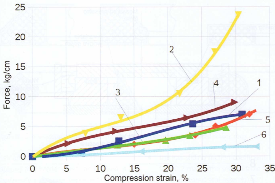
Figure 3. Per-unit force vs compression strain for encapsulated rings with a cross-section of 5.8mm and different rubber core hardnesses and capsule thicknesses: 1, 2 — core hardness Shor A 70; 3, 4 — core hardness Shor A 55; 1, 3 — capsule thickness 0.2 mm; 2, 4 — capsule thickness 0.7 mm; 5 — only core with hardness Shor A 60; 6 — only capsule with thickness 0.4 mm
