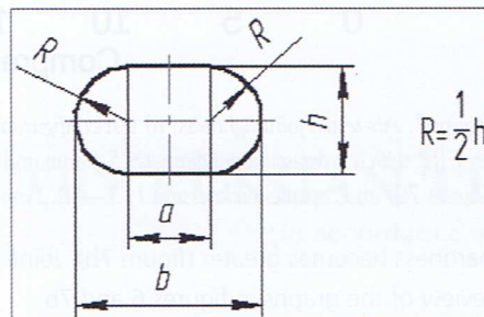
Figure 4. Contact area width calculation
