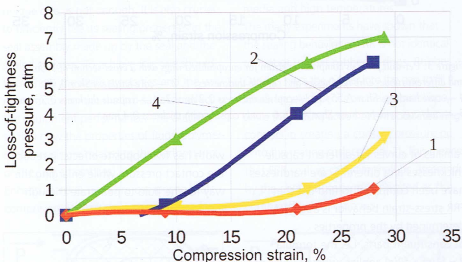
Figure 7. Air-tested joint tightness: a) test configuration; b) compression strain vs loss-of-tightness pressure for FRR with a cross-sectional diameter 5.8 mm and different core hardnesses (1, 2 — Shor A 55; 3, 4 — Shor A 70) and capsule thicknesses (1, 3 — 0.2 mm; 2, 4 — 0.7 mm).
