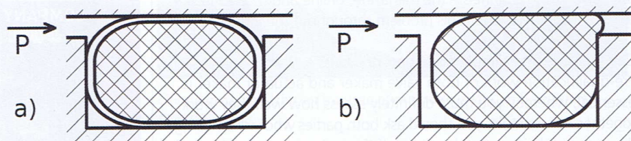
Figure 2. Sealing action of FRR (a) and rubber O-ring (b)
