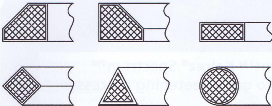
Figure 8. Cross-section configuration options for fluoropolymer-encapsulated sealing rings
