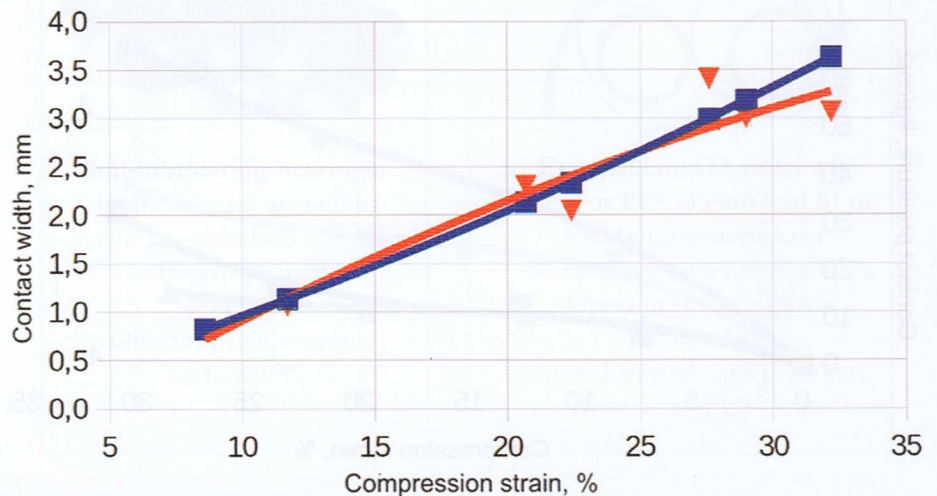
Figure 5. FRR contact area width at different compression strains. Calculation data - ■ vs experimental data - ▼.
